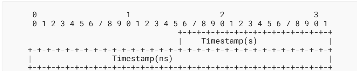
Figure 3: The Timestamp Extended Data Field
