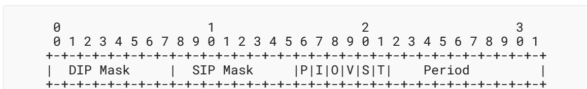
Figure 4: Control Information for Backward Direction Flow Monitoring
