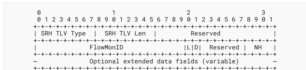
Figure 1: The AltMark SRH TLV for Alternate Marking
