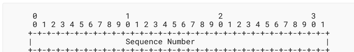
Figure 5: Sequence Number Data Field
