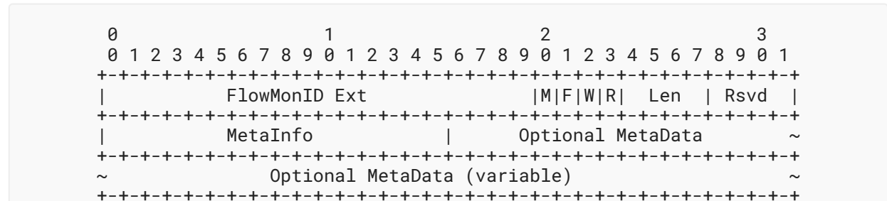
Figure 2: Optional Extended Data Fields for Enhanced Alternate Marking
