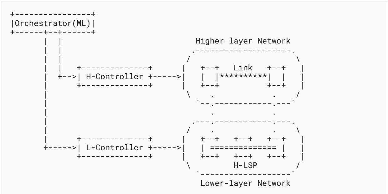
Figure 4: GMPLS-controller Interworking in Multi-Layer Networks
