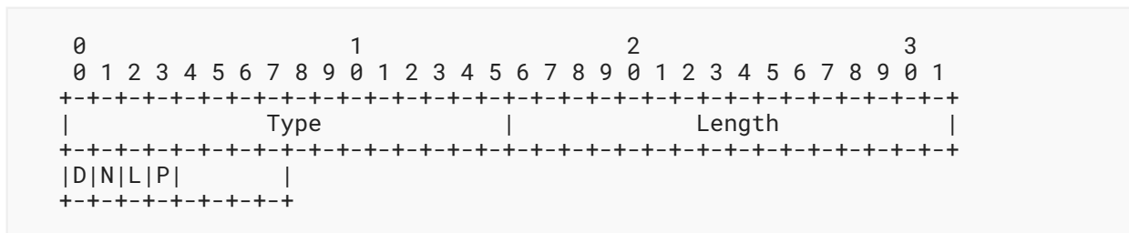
Figure 25: IGP Flag TLV Format
