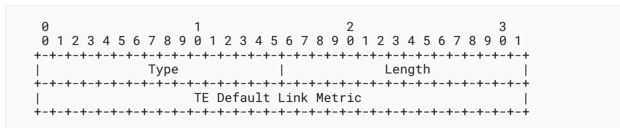
Figure 20: TE Default Metric TLV Format
