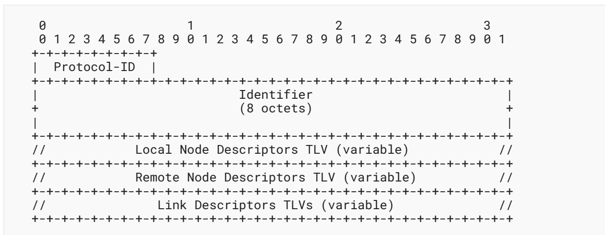
Figure 8: The Link NLRI Format
