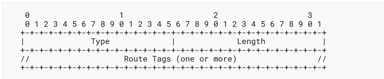
Figure 26: IGP Route Tag TLV Format
