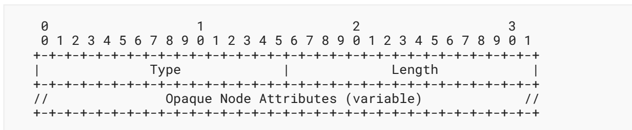
Figure 18: Opaque Node Attribute Format
