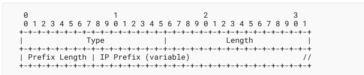
Figure 14: IP Reachability Information TLV Format
