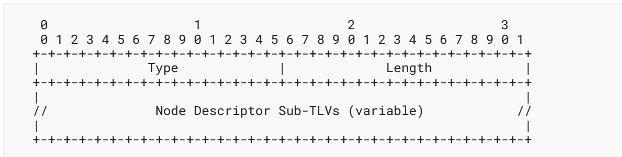
Figure 11: Remote Node Descriptors TLV Format
