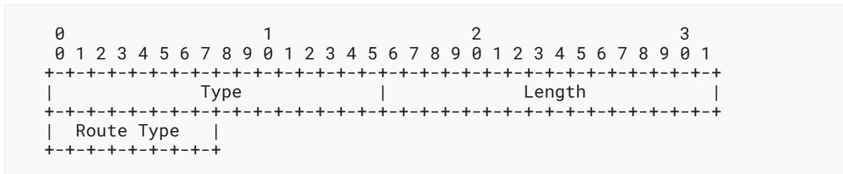
Figure 13: OSPF Route Type TLV Format
