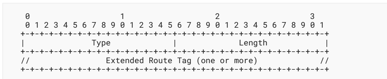
Figure 27: IGP Extended Route Tag TLV Format
