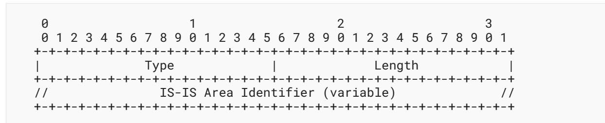
Figure 16: IS-IS Area Identifier TLV Format
