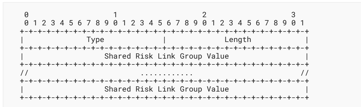
Figure 22: Shared Risk Link Group TLV Format
