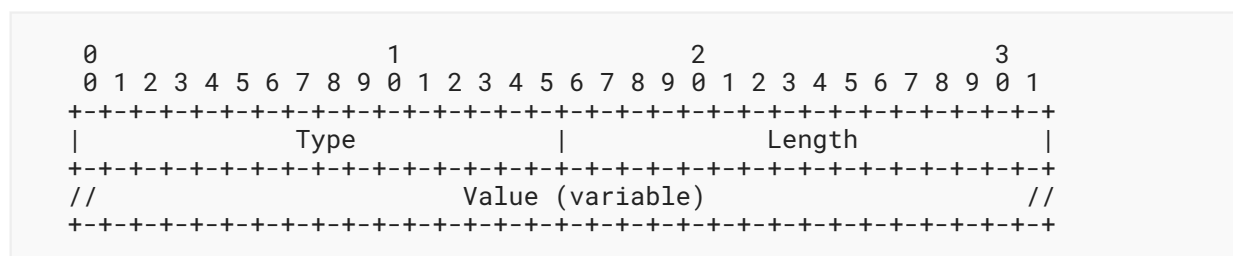
Figure 4: TLV Format
