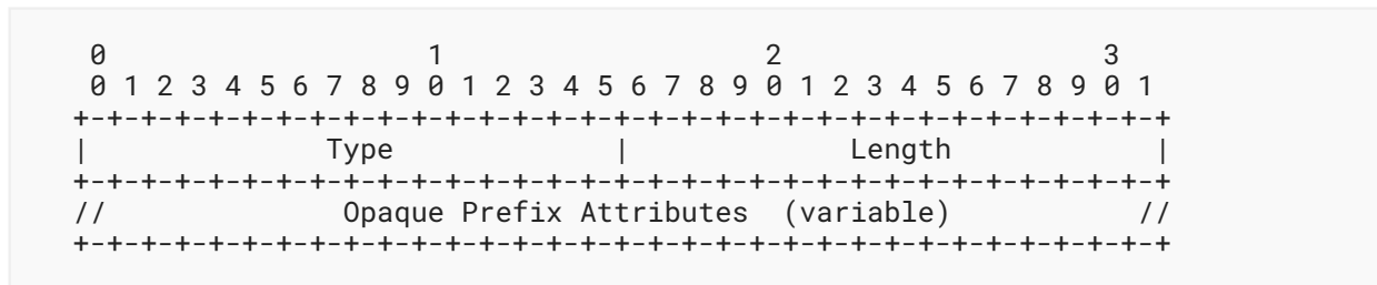
Figure 30: Opaque Prefix Attribute TLV Format
