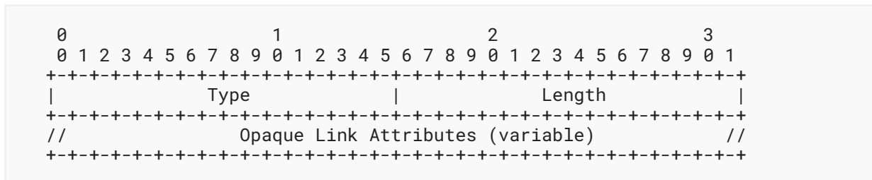
Figure 23: Opaque Link Attribute TLV Format
