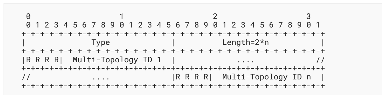
Figure 12: Multi-Topology Identifier TLV Format
