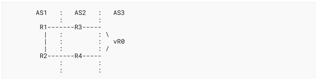
Figure 36: Multi-AS Aggregation
