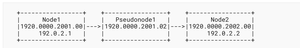
Figure 32: IS-IS Pseudonodes
