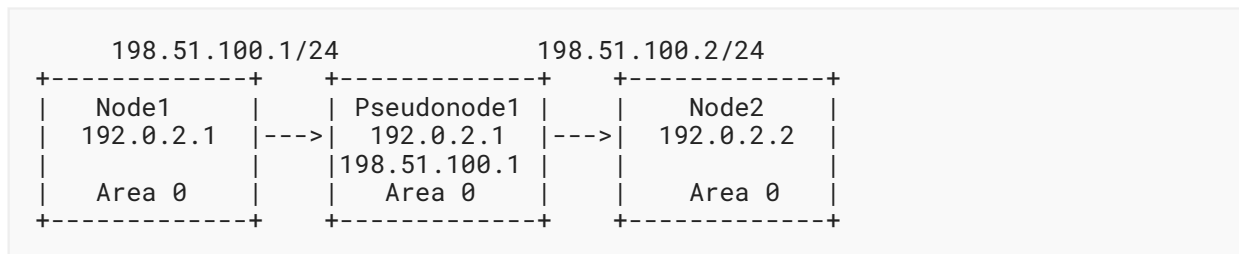
Figure 33: OSPF Pseudonodes
