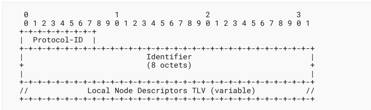
Figure 7: The Node NLRI Format
