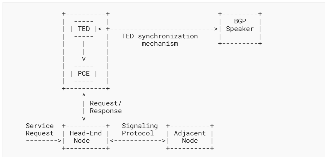
Figure 2: External PCE Node Using a TED Synchronization Mechanism
