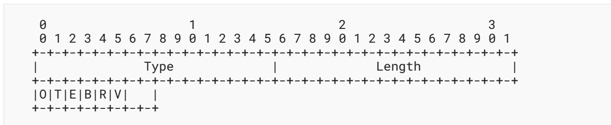
Figure 15: Node Flag Bits TLV Format
