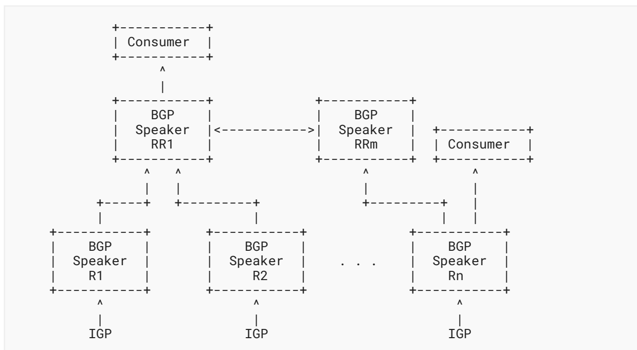
Figure 1: Collection of Link-State and TE Information
