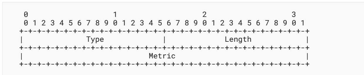
Figure 28: Prefix Metric TLV Format
