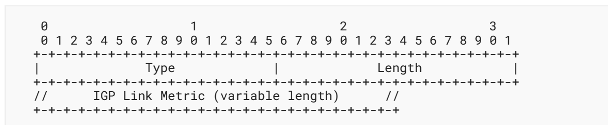
Figure 21: IGP Metric TLV Format
