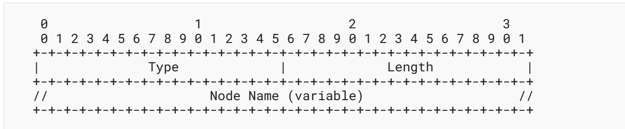
Figure 17: Node Name Format
