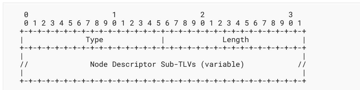
Figure 10: Local Node Descriptors TLV Format
