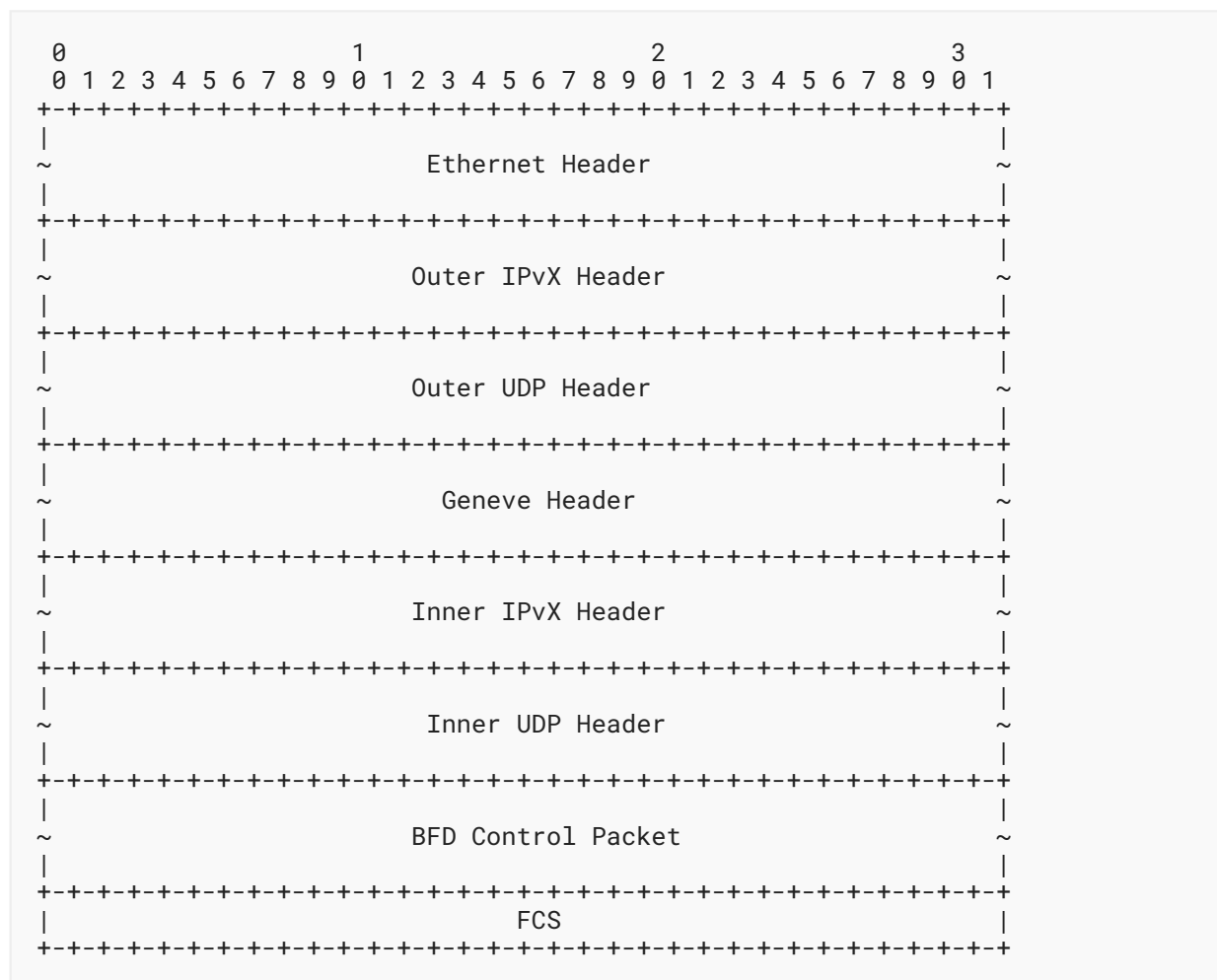
Figure 2: Geneve Encapsulation of a BFD Control Packet with the Inner IP/UDP Header
