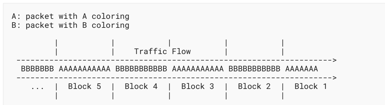
Figure 2: Traffic Coloring
