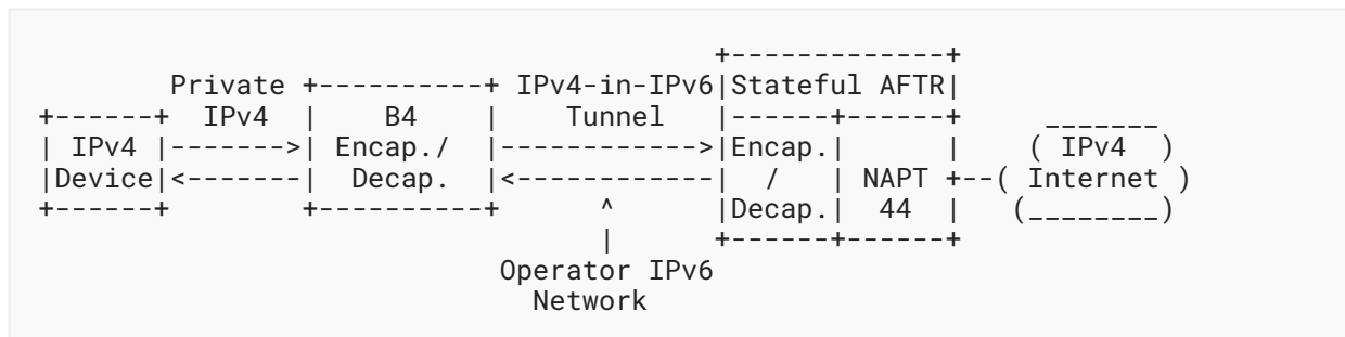
Figure 2: Overview of the DS-Lite Architecture
