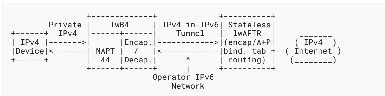
Figure 3: Overview of the lw4o6 Architecture
