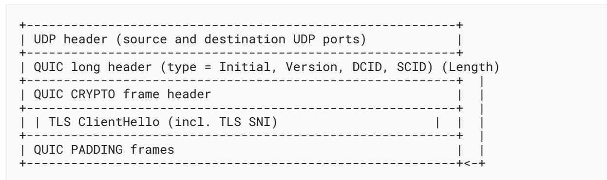
Figure 2: Example Client Initial Datagram Without 0-RTT
