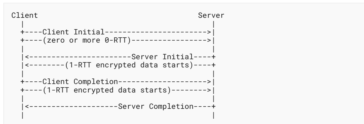
Figure 1: General Communication Pattern Visible in the QUIC Handshake
