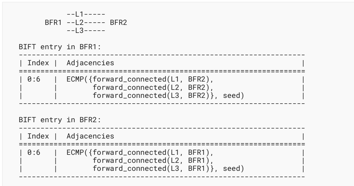
Figure 10: ECMP Example
