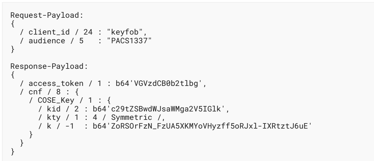
Figure 17: Request and Response Payload for the C Offline
