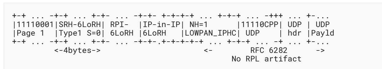
Figure 2: RPI Inserted by the Root in Storing Mode
