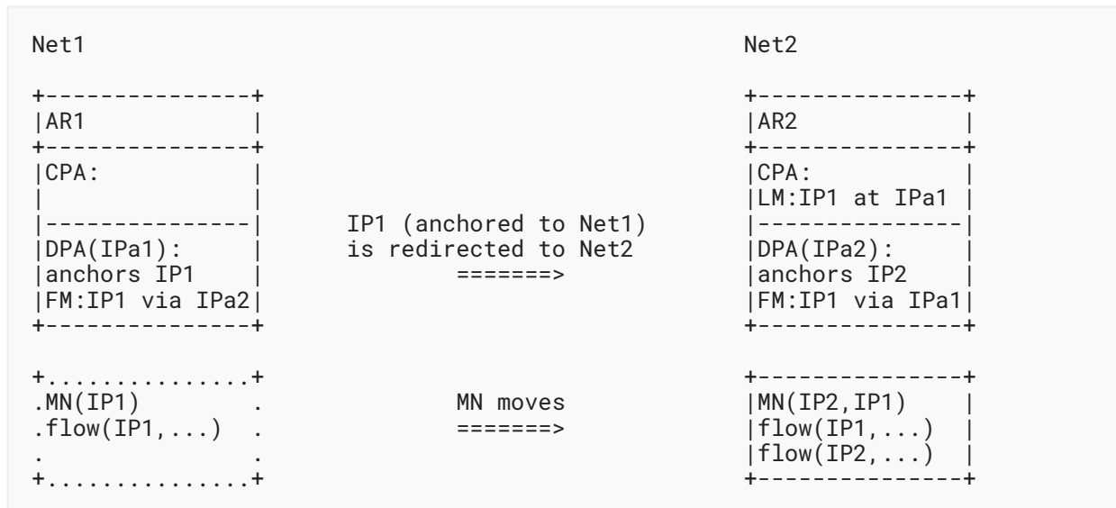
Figure 6: Anchor Redirection
