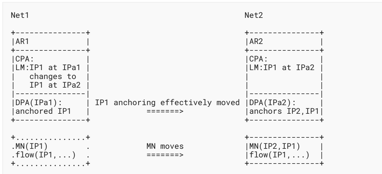
Figure 7: Anchor Relocation
