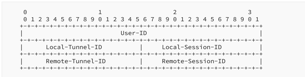
Figure 52: L2TP-LAC Subscriber TLV
