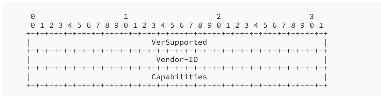
Figure 39: Hello TLV
