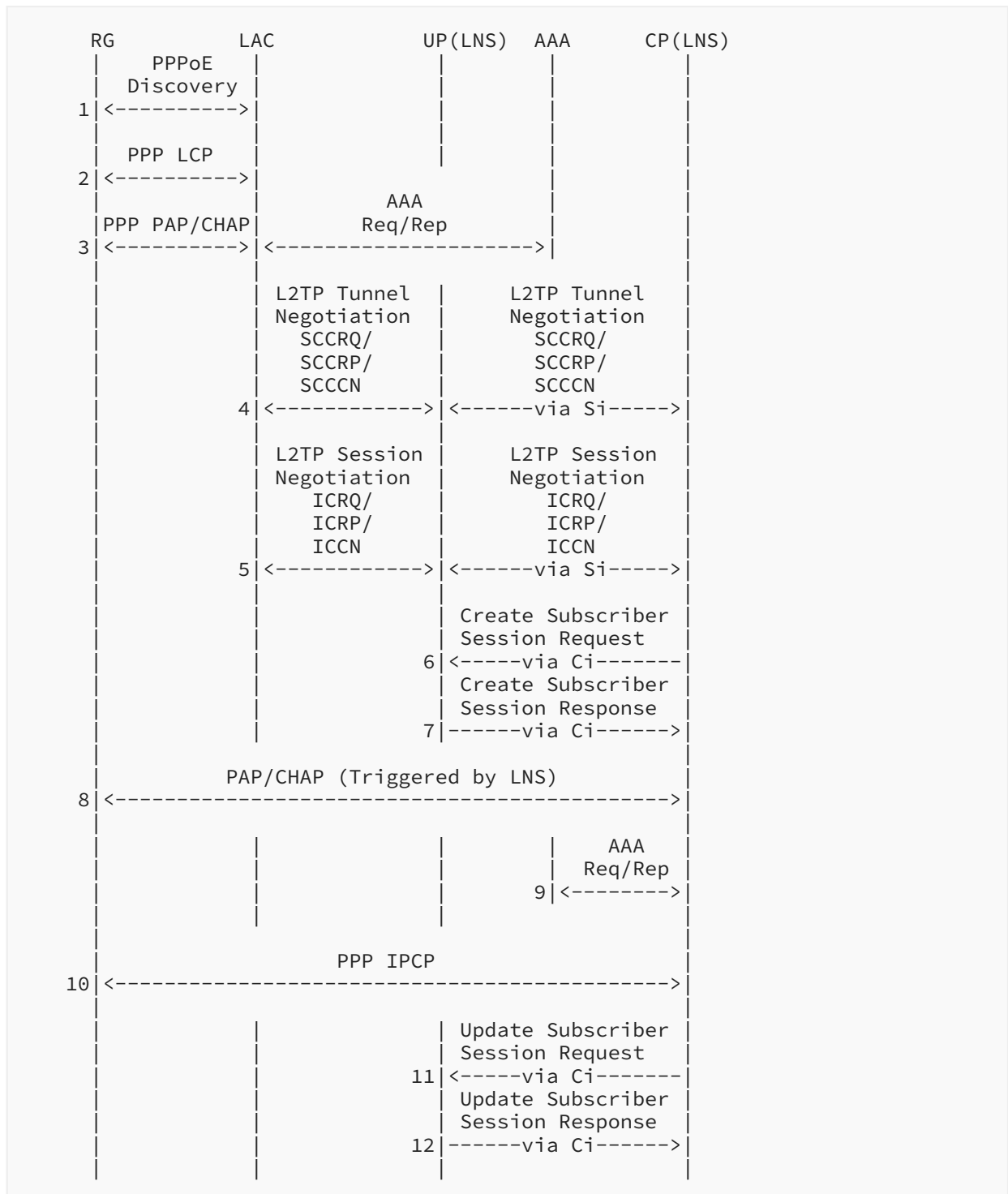
Figure 25: IPv4 L2TP LNS Access
