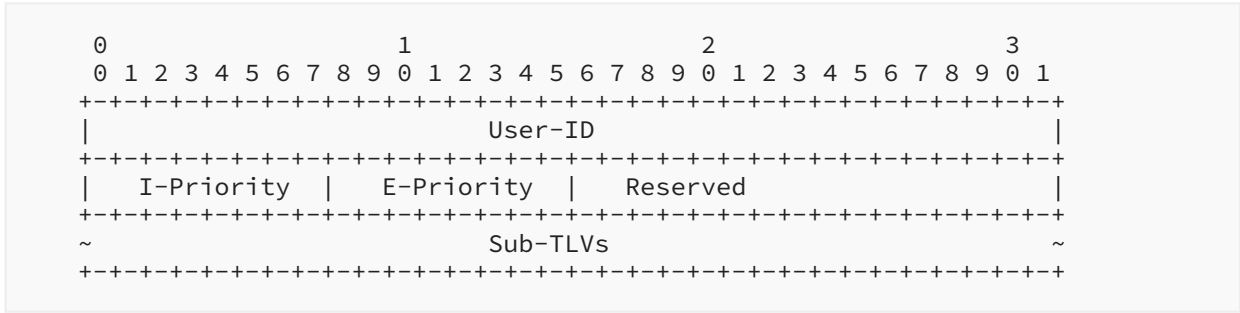
Figure 57: User QoS Policy Information TLV
