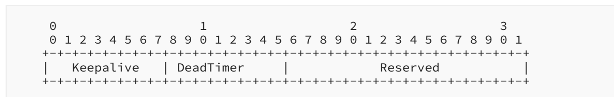
Figure 40: Keepalive TLV
