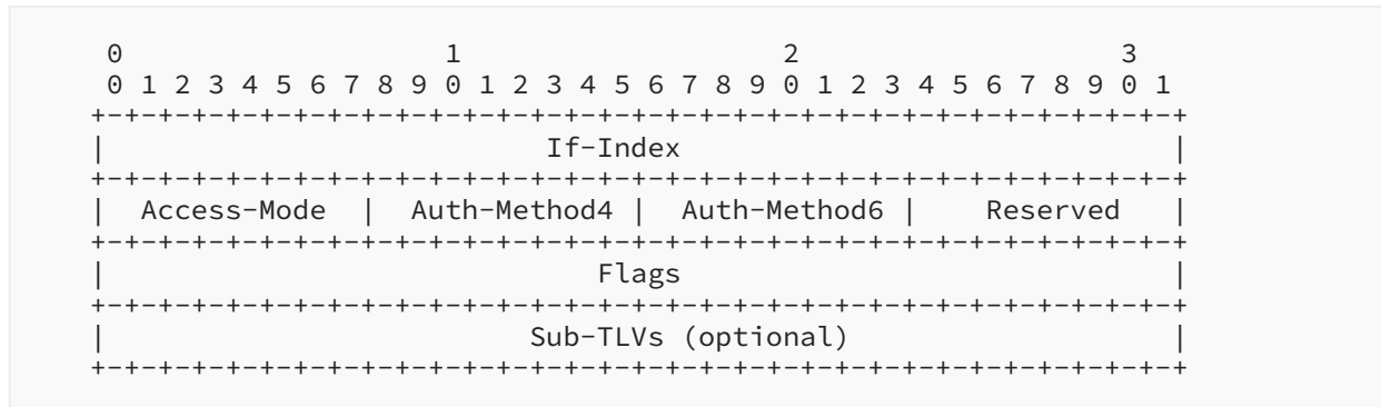
Figure 42: BAS Function TLV
