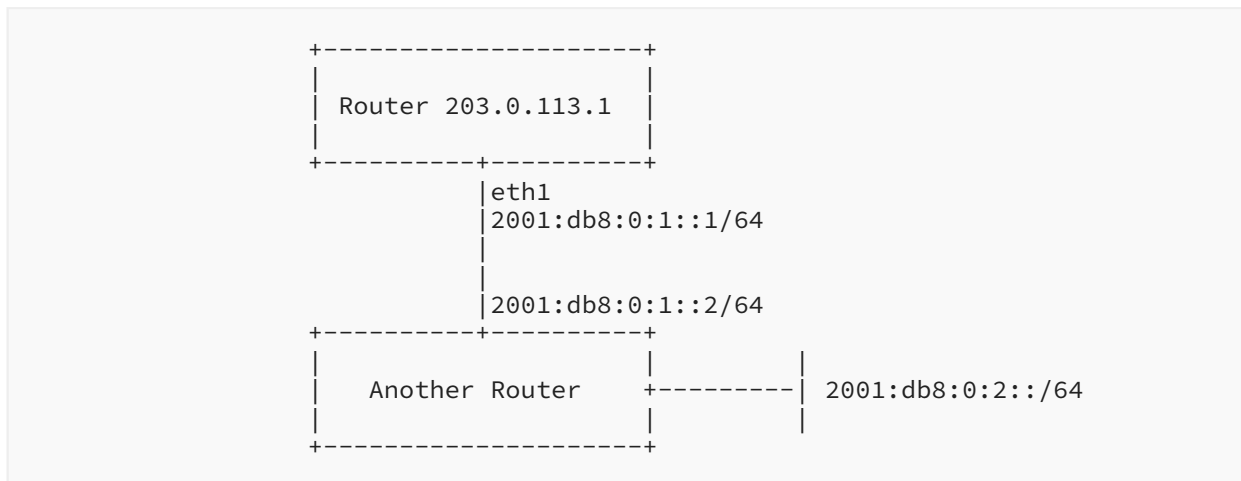
Figure 1: RIPng Example
