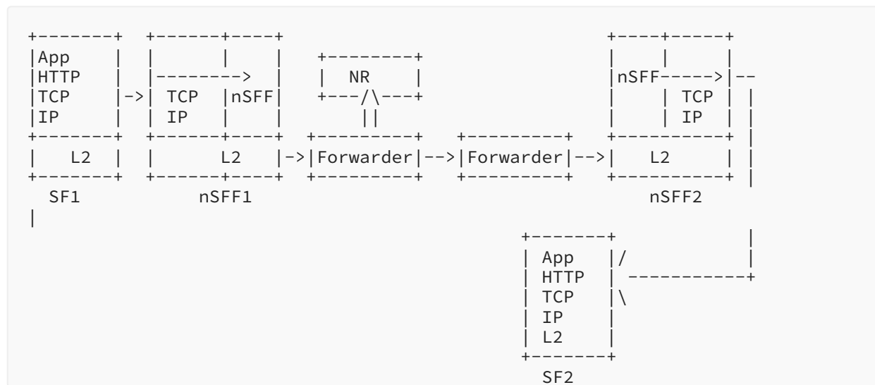
Figure 4: Protocol Layers
