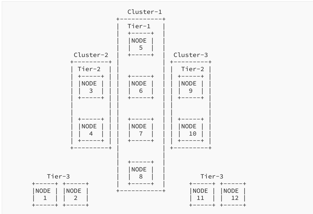
Figure 3: IBGP Sessions with Reflection and Next-Hop-Self
