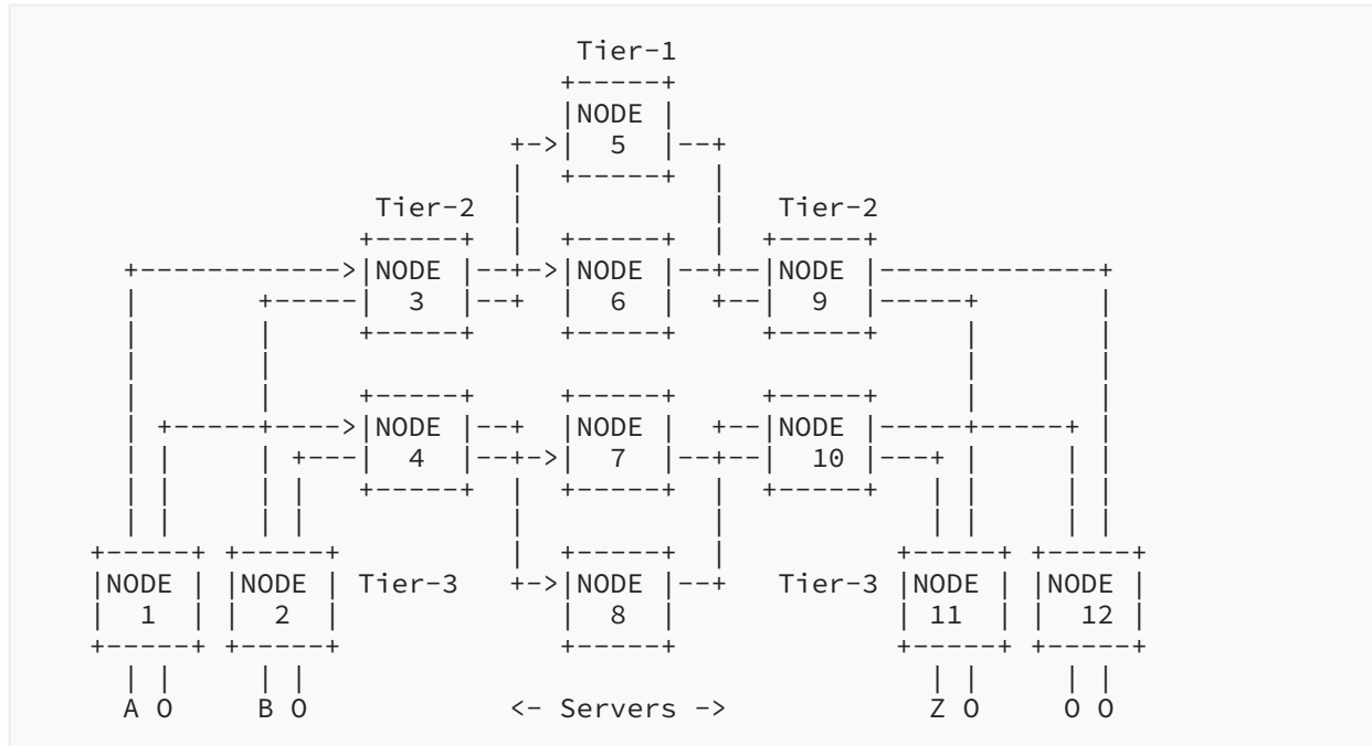
Figure 1: 5-Stage Clos Topology
