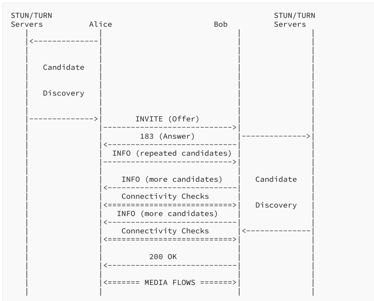
Figure 9: Example of a Typical (Half) Trickle ICE Exchange with SIP
